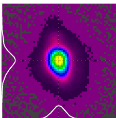
6.45 \mu\text{m} output beam profile of the ZGP RISTRA OPO at \sim 5 mJ pulse energy
