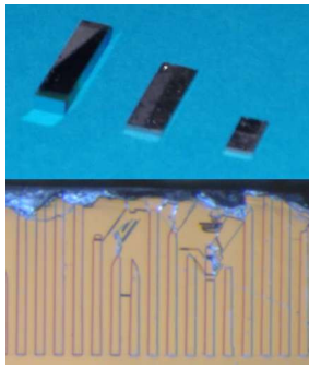
Thick OP-GaAs crystals for mid-IR frequency conversion
